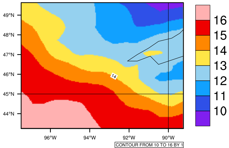
Yearly tasmax (c) In 1975-2005 MIROC4h historical - Minnesota
