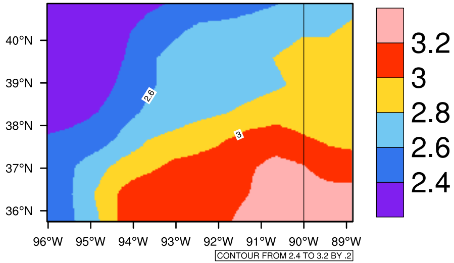
Yearly pr (mm/day) In 2020-2029 MIROC4h RCP45 - Missouri
