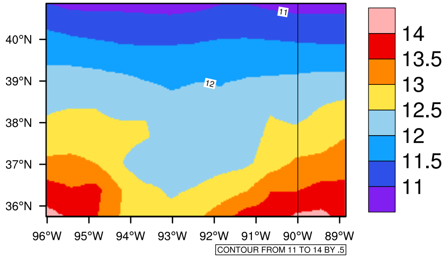
Yearly tasmin (c) In 2020-2029 MIROC4h RCP45 - Missouri
