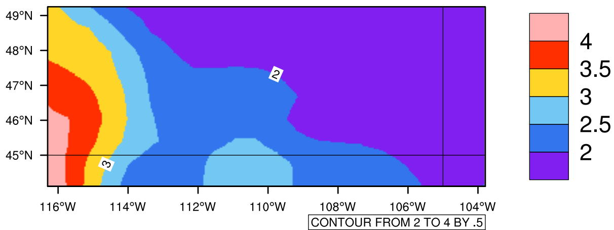
Yearly pr (mm/day) In 2020-2029 MIROC4h RCP45 - Montana
