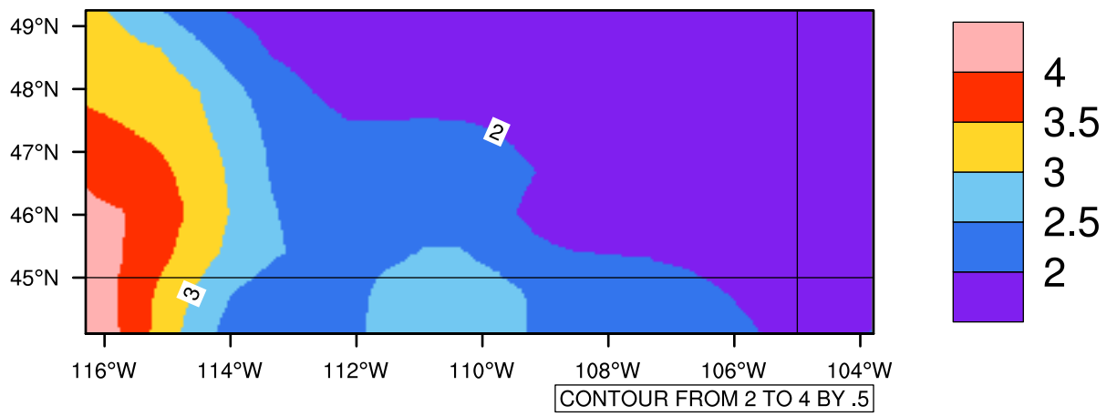
Yearly pr (mm/day) In 2020-2029 MIROC4h RCP45 - Montana
