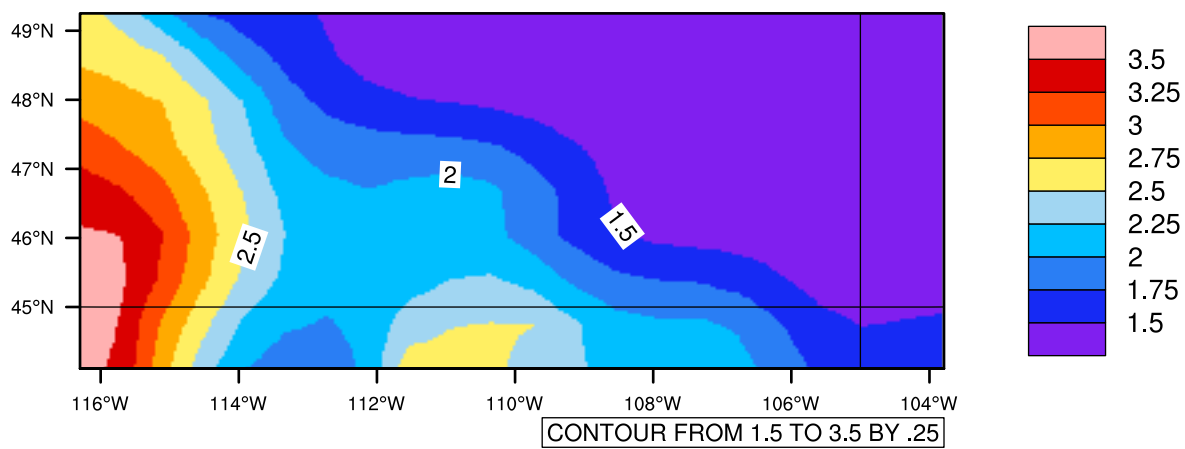
Yearly pr (mm/day) In 1975-2005 MIROC4h historical - Montana
