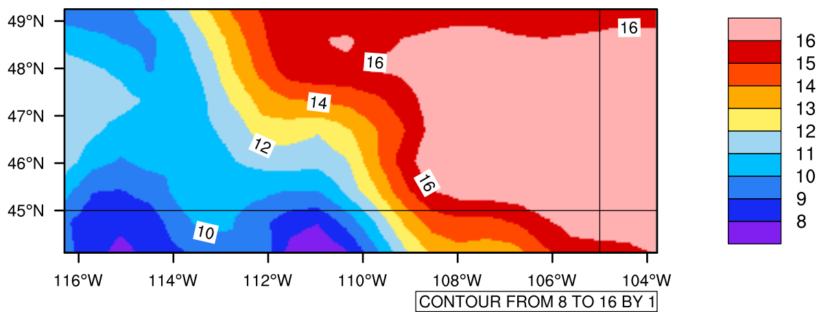
Yearly tasmax (c) In 2020-2029 MIROC4h RCP45 - Montana
