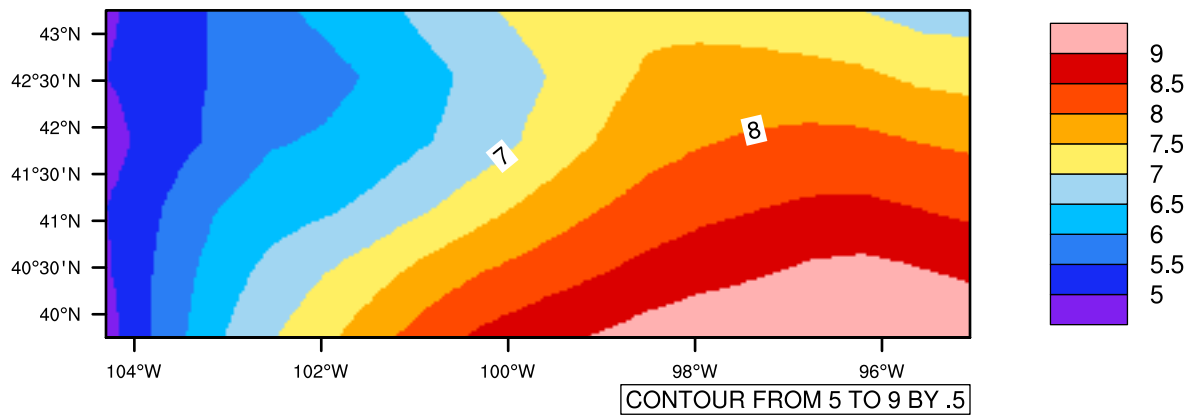
Yearly tasmin (c) In 1975-2005 MIROC4h historical - Nebraska
