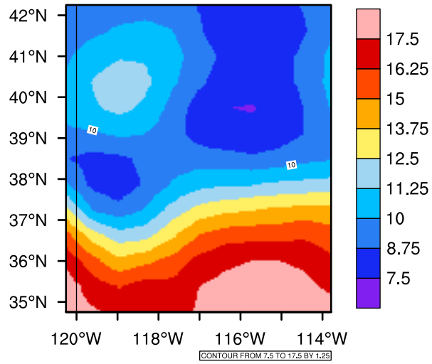
Yearly tas (c) In 2020-2029 MIROC4h RCP45 - Nevada
