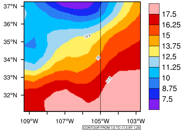
Yearly tas (c) In 2020-2029 MIROC4h RCP45 - New Mexico
