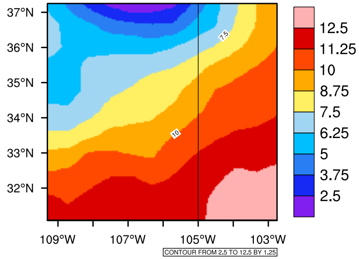
Yearly tasmin (c) In 2020-2029 MIROC4h RCP45 - New Mexico
