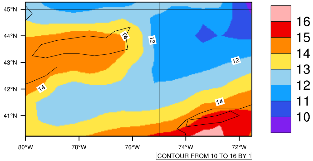
Yearly tasmax (c) In 1975-2005 MIROC4h historical - New York
