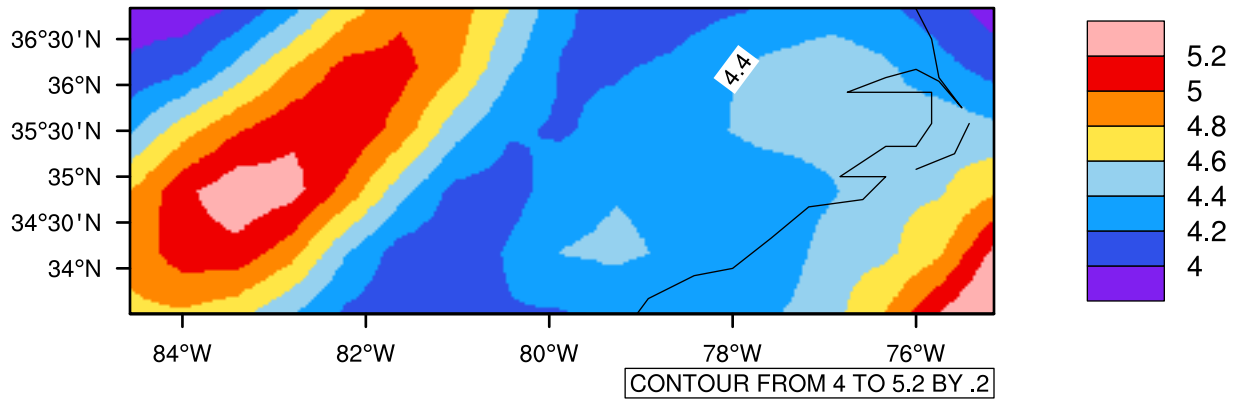
Yearly pr (mm/day) In 2020-2029 MIROC4h RCP45 - North Carolina
