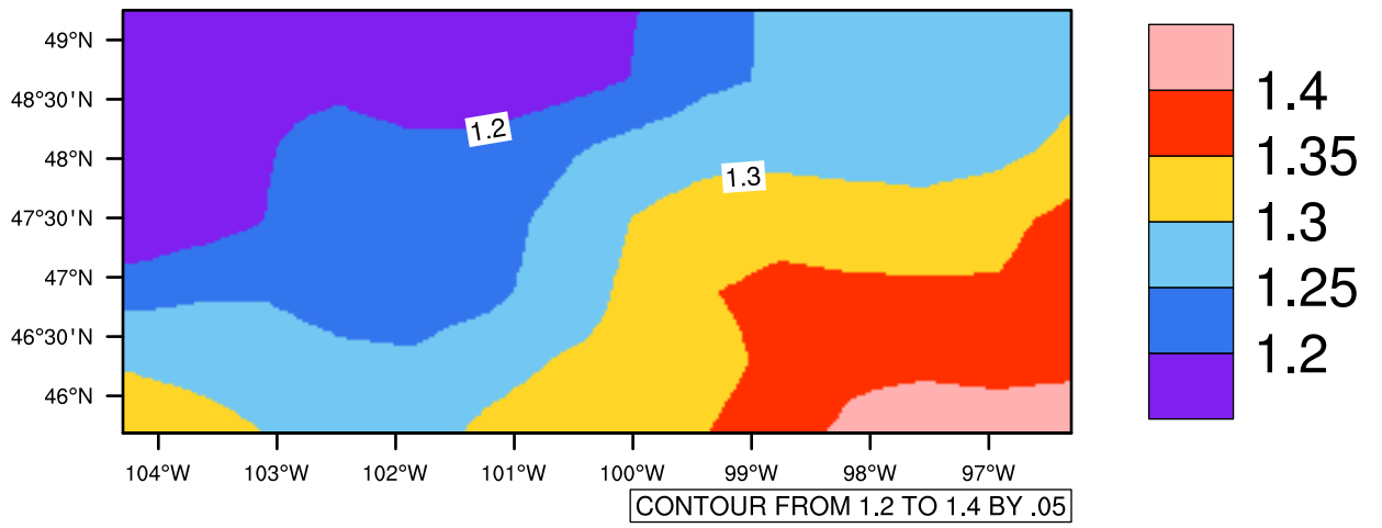
Yearly pr (mm/day) In 1975-2005 MIROC4h historical - North Dakota
