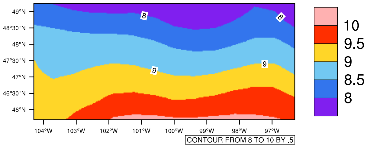
Yearly tas (c) In 1975-2005 MIROC4h historical - North Dakota
