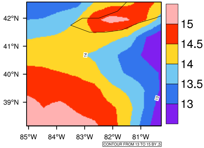
Yearly tas (c) In 2020-2029 MIROC4h RCP45 - Ohio
