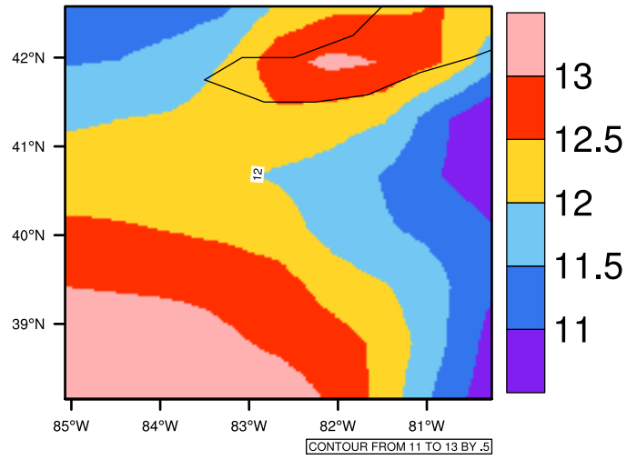
Yearly tas (c) In 1975-2005 MIROC4h historical - Ohio
