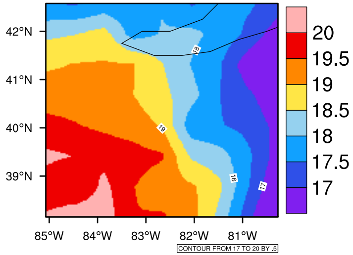
Yearly tasmax (c) In 2020-2029 MIROC4h RCP45 - Ohio
