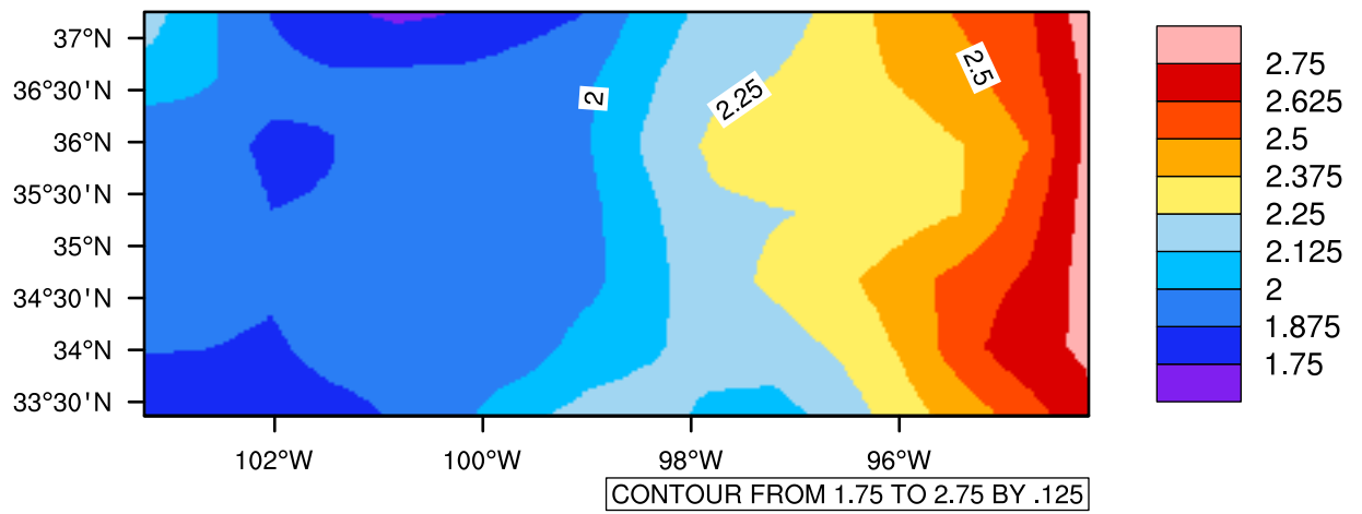
Yearly pr (mm/day) In 2020-2029 MIROC4h RCP45 - Oklahoma
