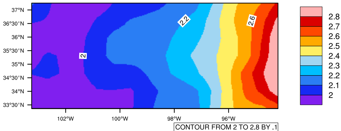
Yearly pr (mm/day) In 1975-2005 MIROC4h historical - Oklahoma
