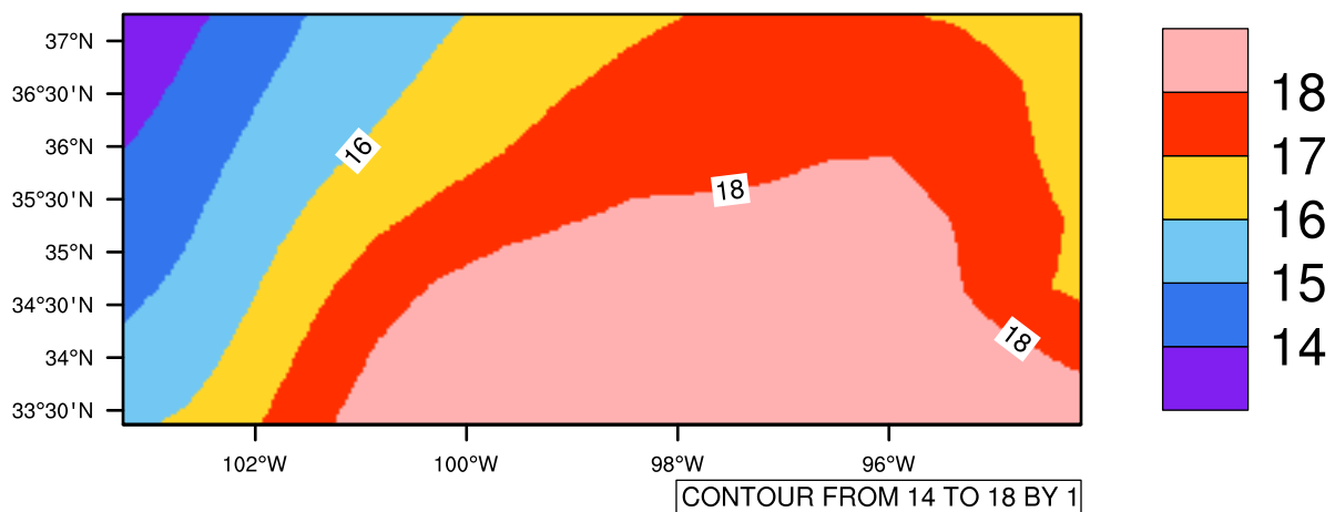
Yearly tas (c) In 1975-2005 MIROC4h historical - Oklahoma
