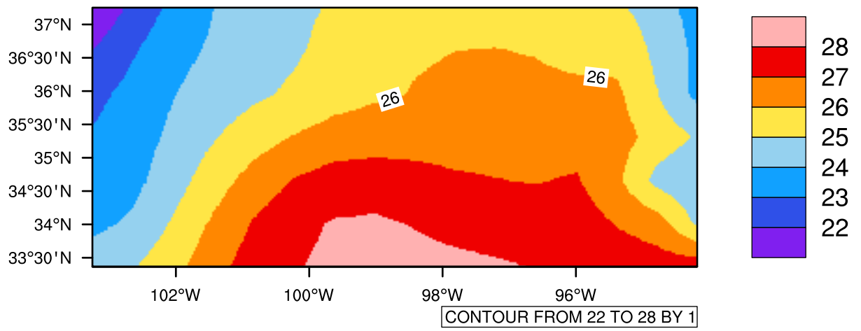
Yearly tasmax (c) In 2020-2029 MIROC4h RCP45 - Oklahoma
