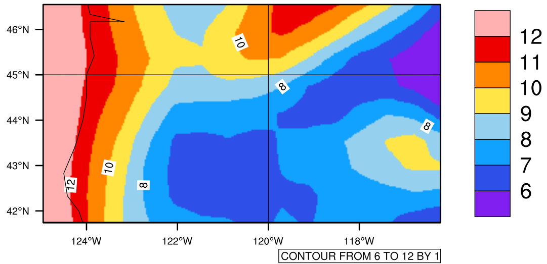
Yearly tas (c) In 1975-2005 MIROC4h historical - Oregon
