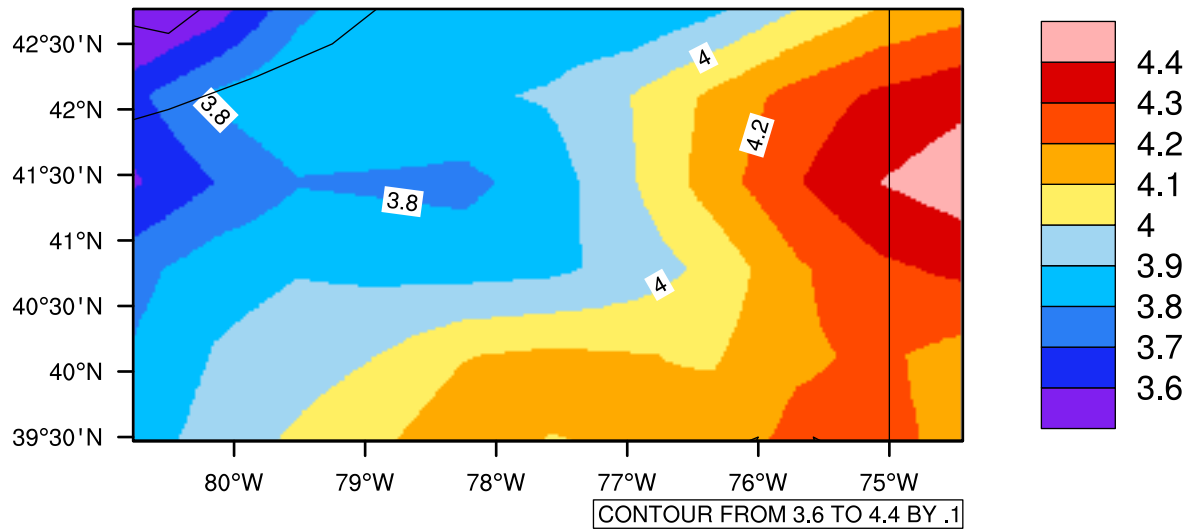
Yearly pr (mm/day) In 2020-2029 MIROC4h RCP45 - Pennsylvania
