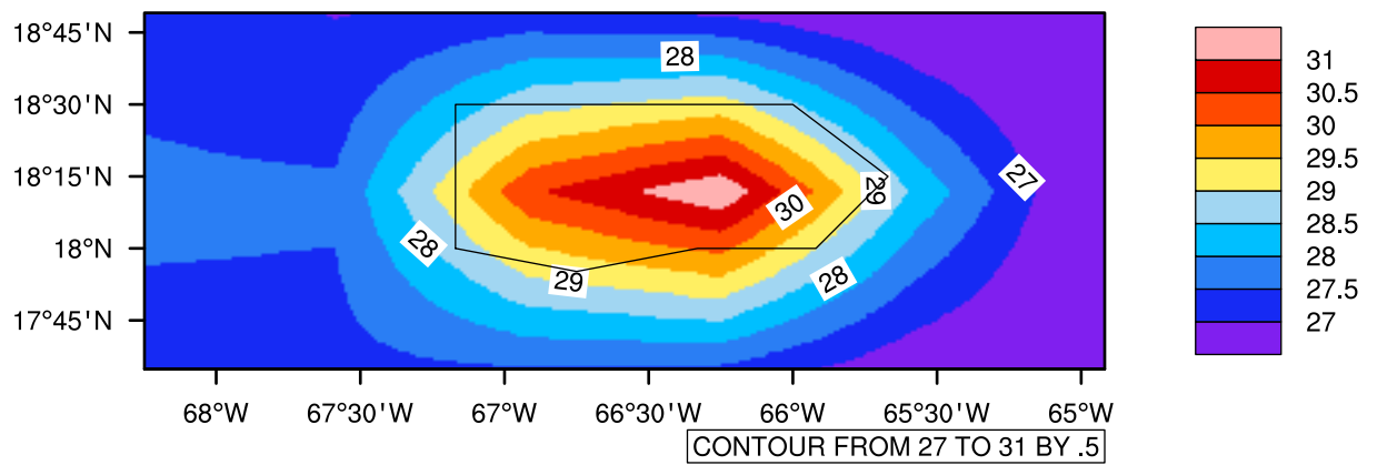
Yearly tasmax (c) In 2020-2029 MIROC4h RCP45 - Puerto Rico
