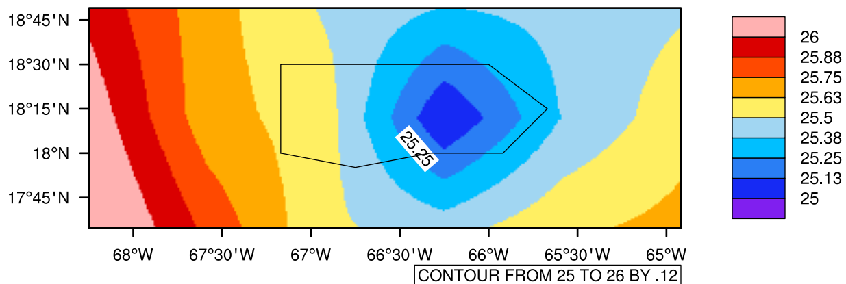
Yearly tasmin (c) In 2020-2029 MIROC4h RCP45 - Puerto Rico
