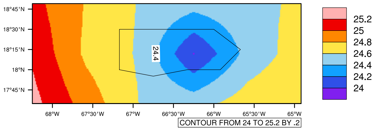
Yearly tasmin (c) In 1975-2005 MIROC4h historical - Puerto Rico
