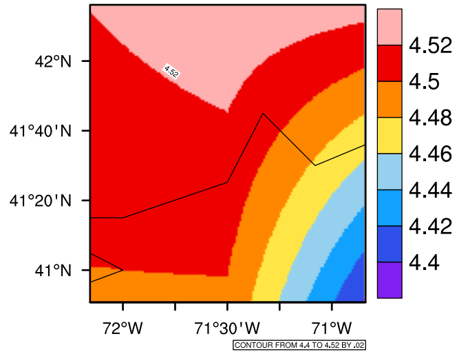
Yearly pr (mm/day) In 2020-2029 MIROC4h RCP45 - Rhode Island
