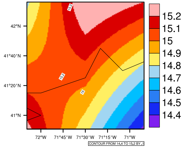
Yearly tasmx (c) In 1975-2005 MIROC4h historical - Rhode Island
