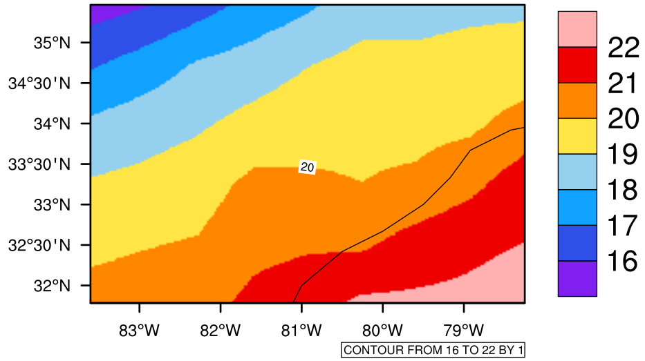
Yearly tas (c) In 2020-2029 MIROC4h RCP45 - South Carolina
