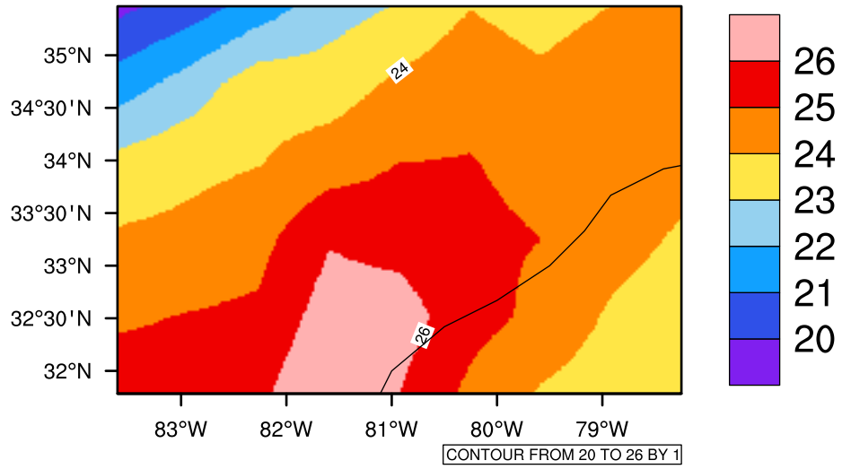
Yearly tasmax (c) In 2020-2029 MIROC4h RCP45 - South Carolina
