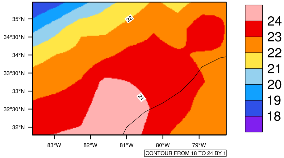
Yearly tasmax (c) In 1975-2005 MIROC4h historical - South Carolina
