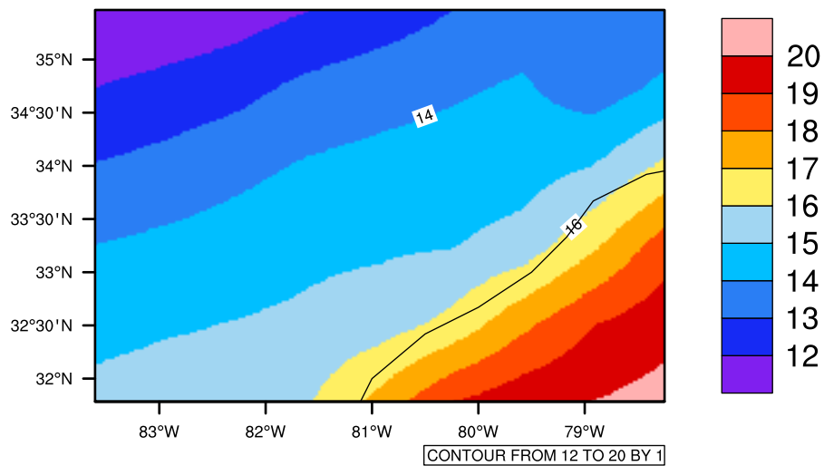
Yearly tasmin (c) In 1975-2005 MIROC4h historical - South Carolina
