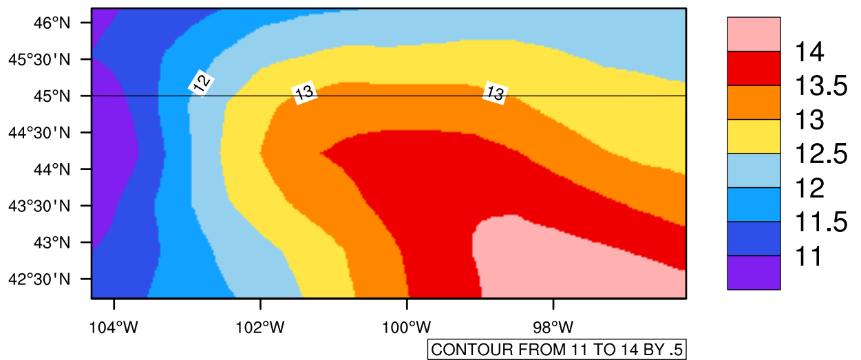
Yearly tas (c) In 2020-2029 MIROC4h RCP45 - South Dakota
