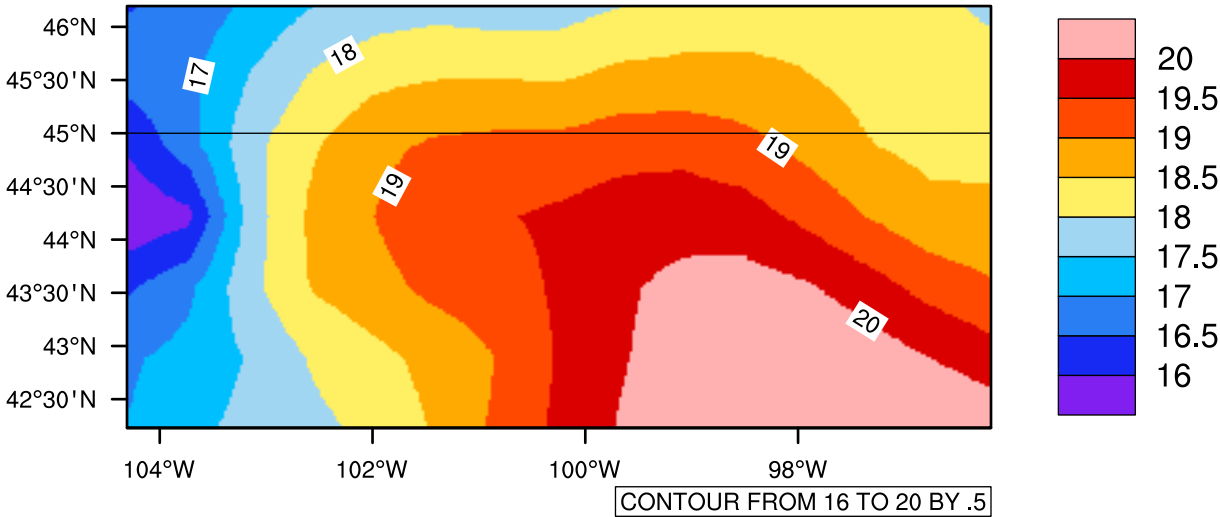
Yearly tasmax (c) In 2020-2029 MIROC4h RCP45 - South Dakota
