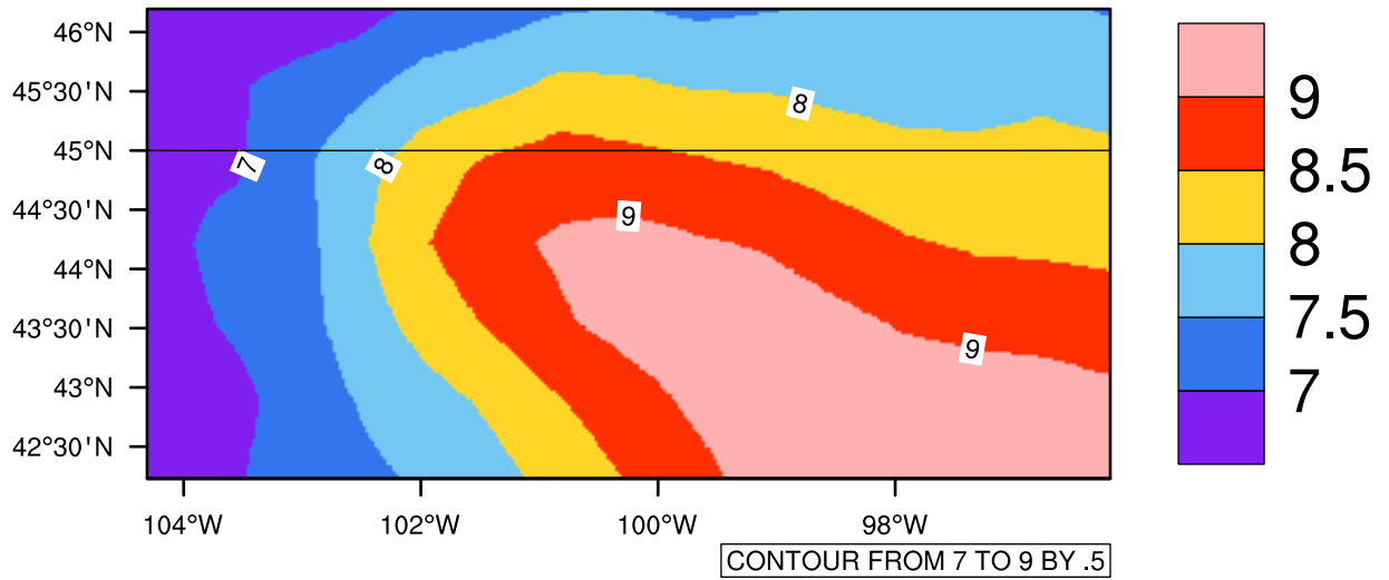
Yearly tasmin (c) In 2020-2029 MIROC4h RCP45 - South Dakota
