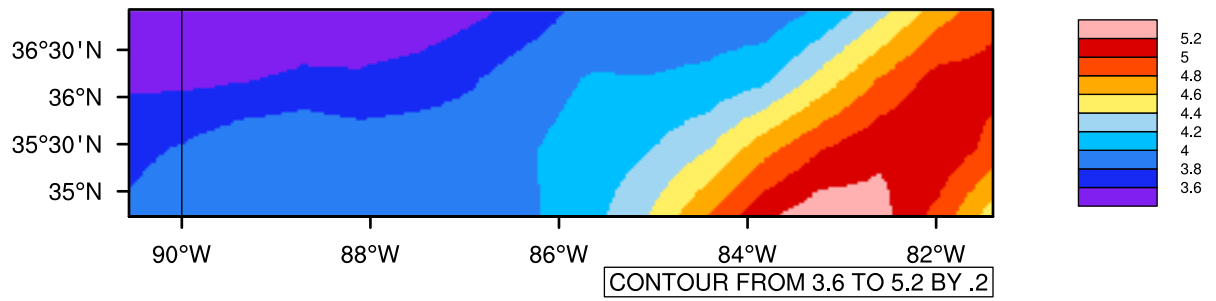
Yearly pr (mm/day) In 2020-2029 MIROC4h RCP45 - Tennessee
