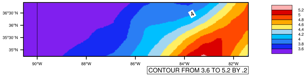
Yearly pr (mm/day) In 1975-2005 MIROC4h historical - Tennessee
