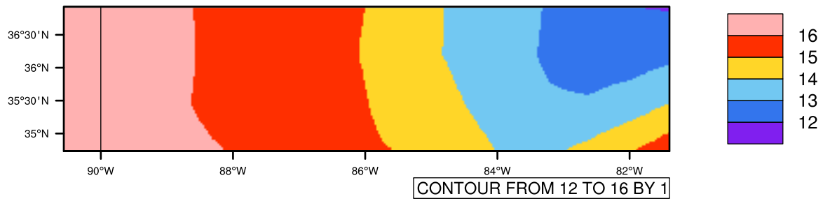
Yearly tas (c) In 1975-2005 MIROC4h historical - Tennessee
