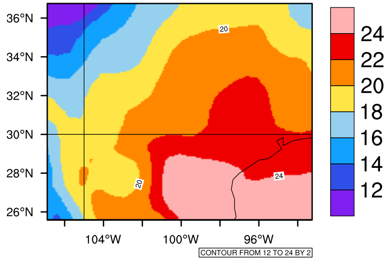
Yearly tas (c) In 2020-2029 MIROC4h RCP45 - Texas
