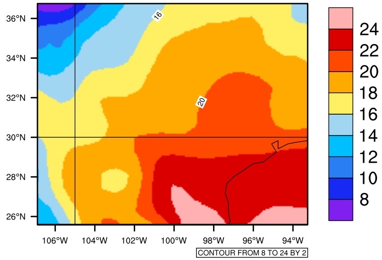
Yearly tas (c) In 1975-2005 MIROC4h historical - Texas
