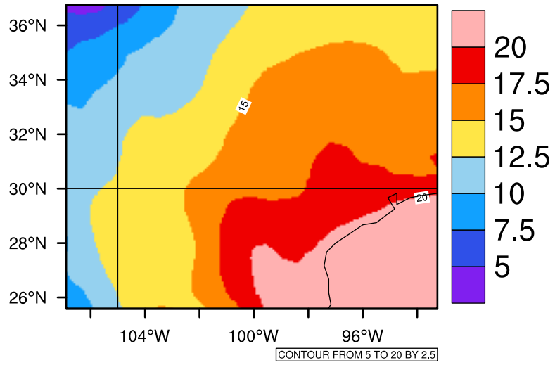
Yearly tasmin (c) In 2020-2029 MIROC4h RCP45 - Texas
