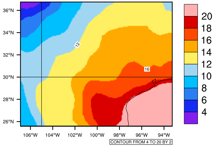
Yearly tasmin (c) In 1975-2005 MIROC4h historical - Texas
