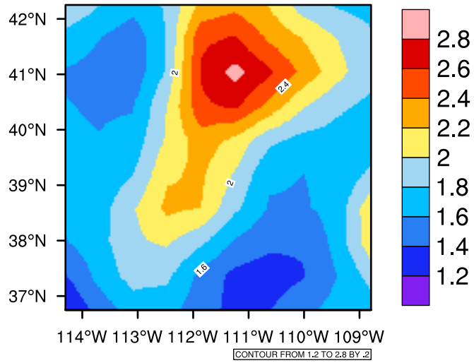
Yearly pr (mm/day) In 2020-2029 MIROC4h RCP45 - Utah
