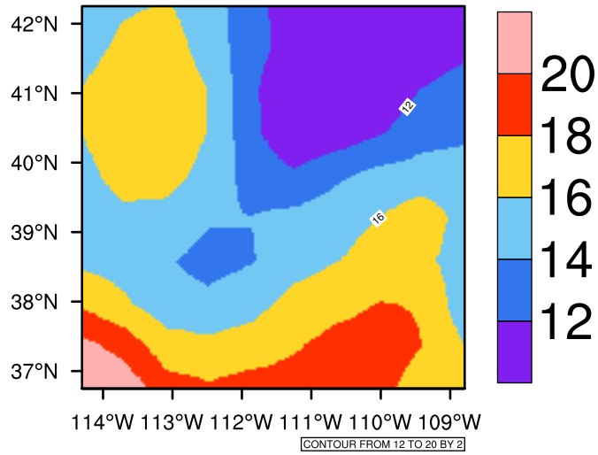
Yearly tasmx (c) In 2020-2029 MIROC4h RCP45 - Utah
