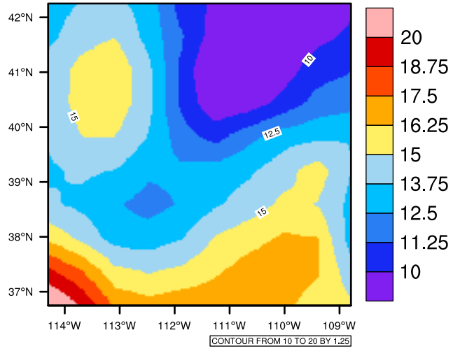
Yearly tasmax (c) In 1975-2005 MIROC4h historical - Utah
