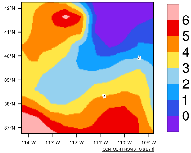
Yearly tasmin (c) In 1975-2005 MIROC4h historical - Utah
