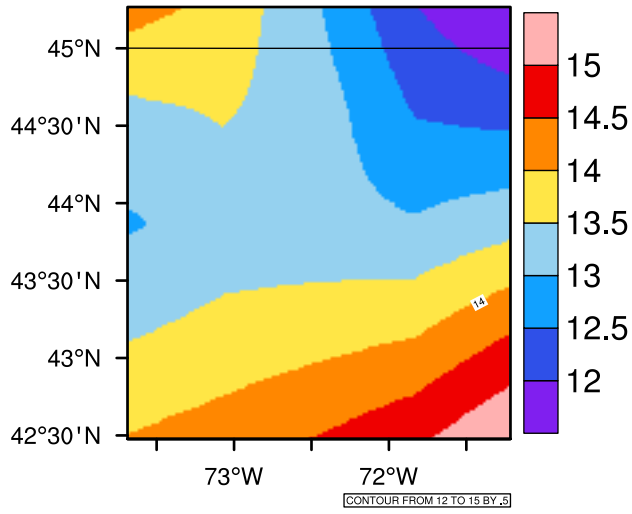
Yearly tasmax (c) In 2020-2029 MIROC4h RCP45 - Vermont
