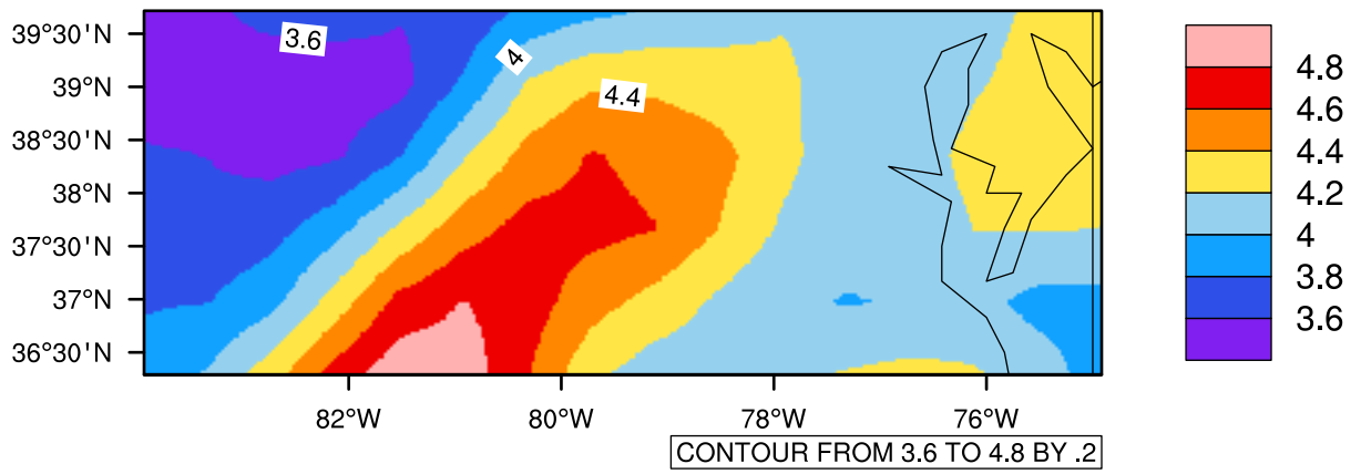
Yearly pr (mm/day) In 2020-2029 MIROC4h RCP45 - Virginia
