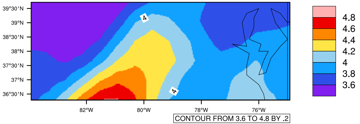
Yearly pr (mm/day) In 1975-2005 MIROC4h historical - Virginia
