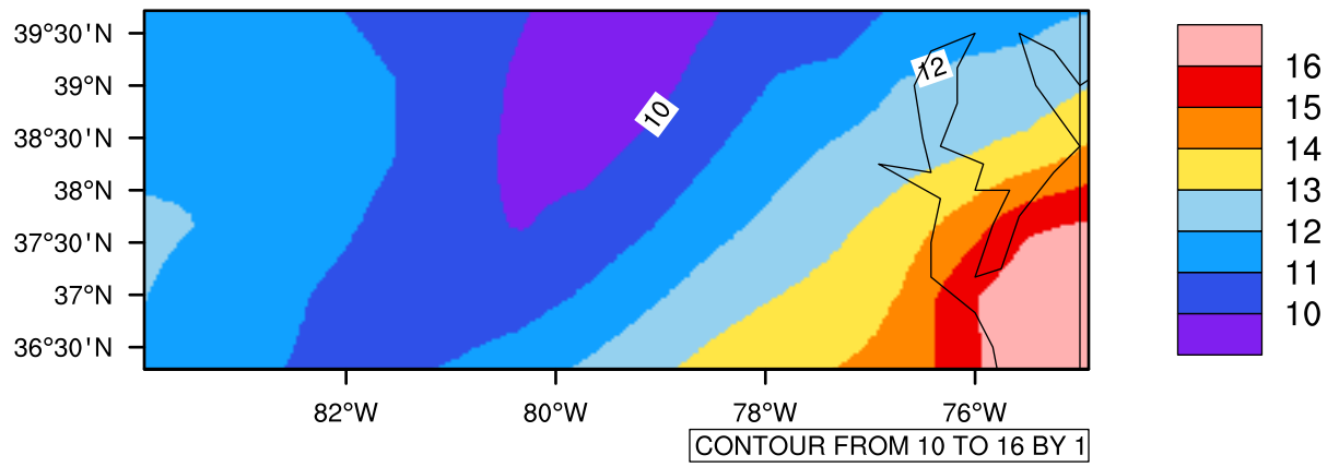
Yearly tasmin (c) In 2020-2029 MIROC4h RCP45 - Virginia
